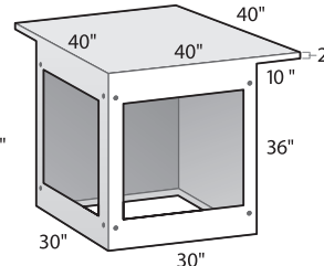
90° CORNER UNIT W/ 2 SIDE CANTILEVERS LOC1C
