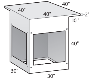
90° BAR-HEIGHT CORNER UNIT W/ 2 SIDE 10" CANTILEVERS LOC1CT
