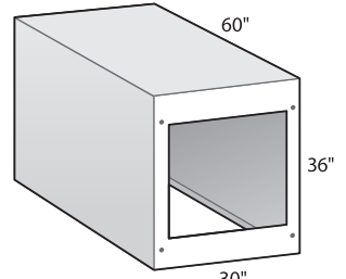
60" UNIT LOC60
