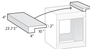
STRAIGHT RAISED BACKSPASH LOC10RBS
