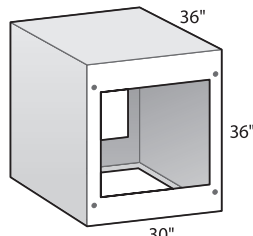
36" UNIT LOC36
