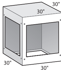
90° CORNER UNIT LOC1
