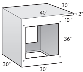
30" UNIT W/ 10" CANTILEVER BACKSIDE LOC30C
