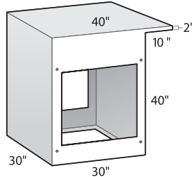
30" BAR-HEIGHT UNIT W/ 10" CANTILEVER BACKSIDE LOC30CT
